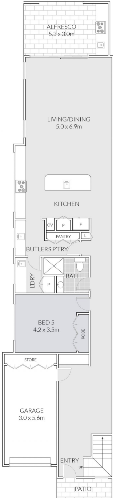
GROUND FLOOR
