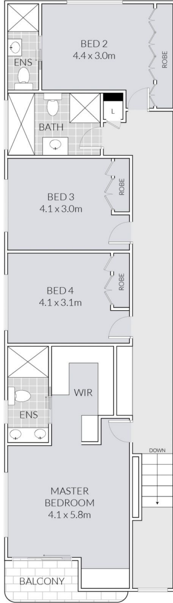
FIRST FLOOR
