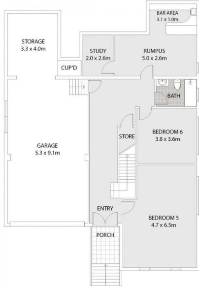
MAIN FLOOR
