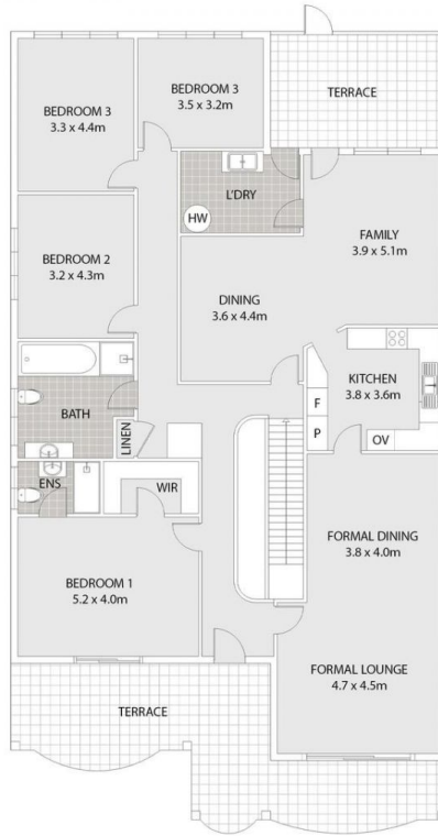
UPPER FLOOR
