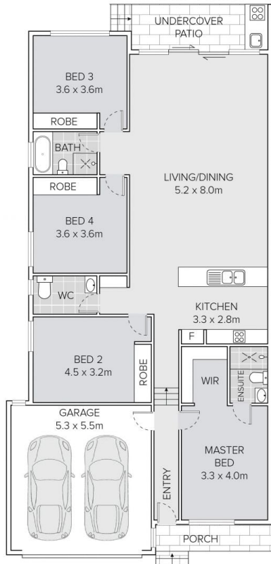
FLOOR PLAN
